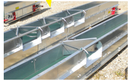
Distribution gate with cable control
